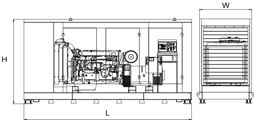
Generator with Soundproof Canopy
