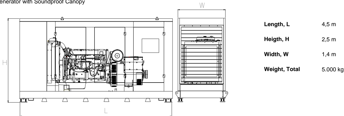
Generator with Soundproof Canopy
