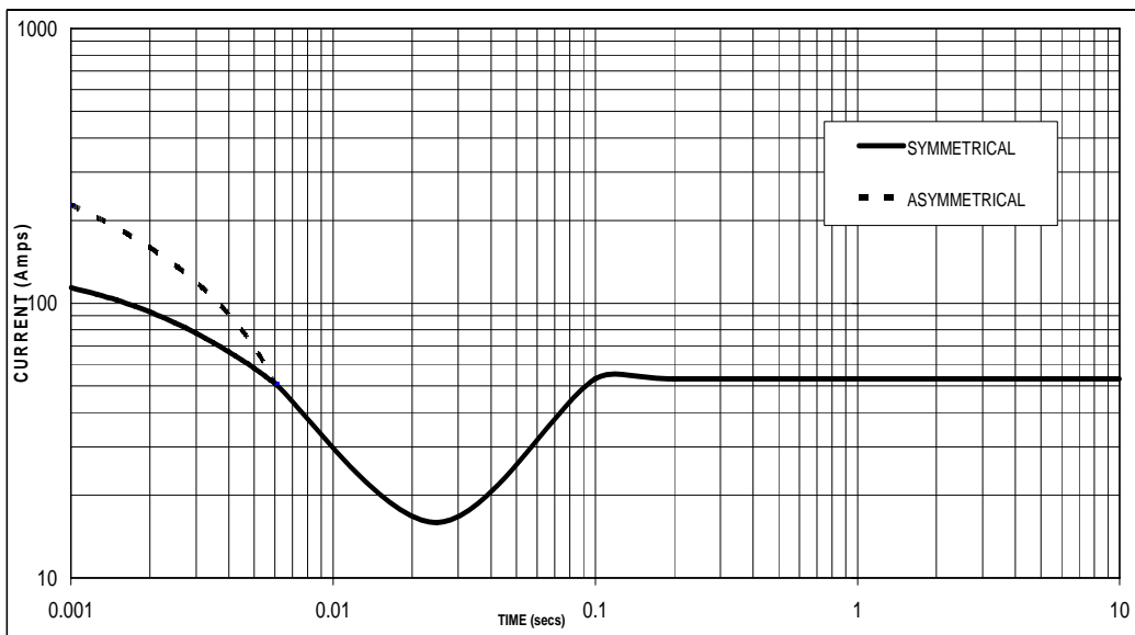
Sustained Short Circuit = 53 Amps
