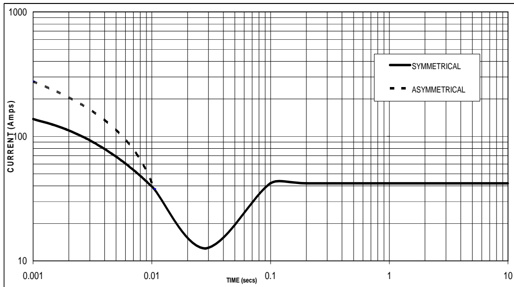
Sustained Short Circuit = 42 Amps
