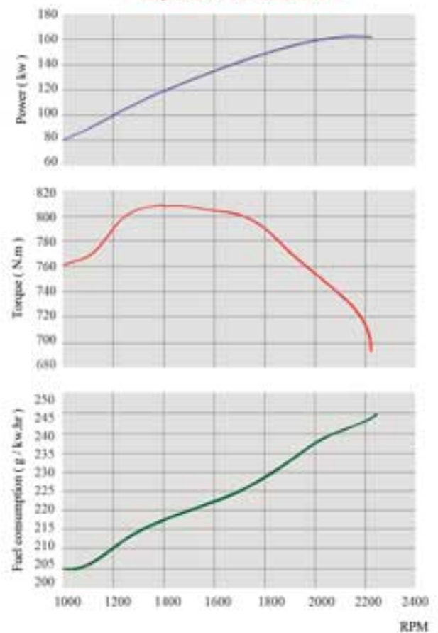
Output power , torque and fuel consumption according to 80/1269 EEC Standard
